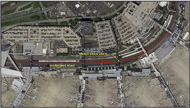
Departures Road Trench Drain Survey at Philadelphia International Airport (PHL)
